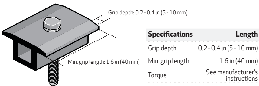
Fig. 1: Clamp specifications
