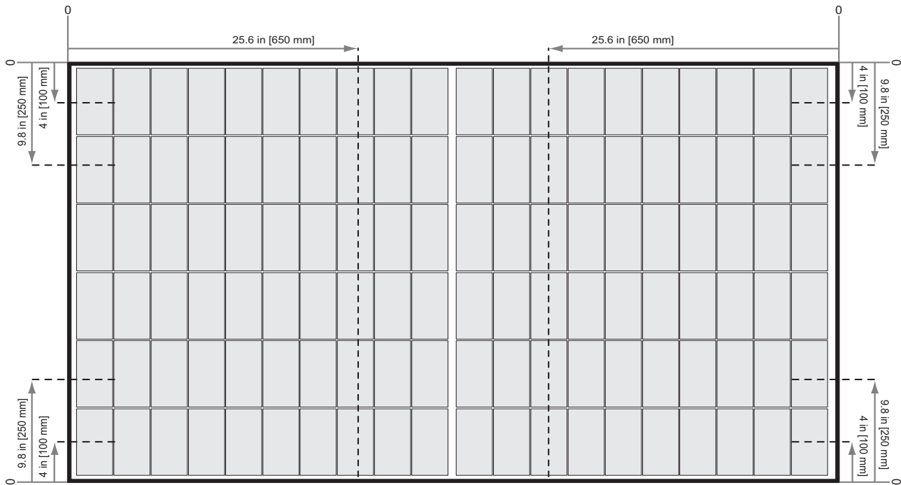
Fig. 4: Clamping of panels with rails parallel to long side of the module
