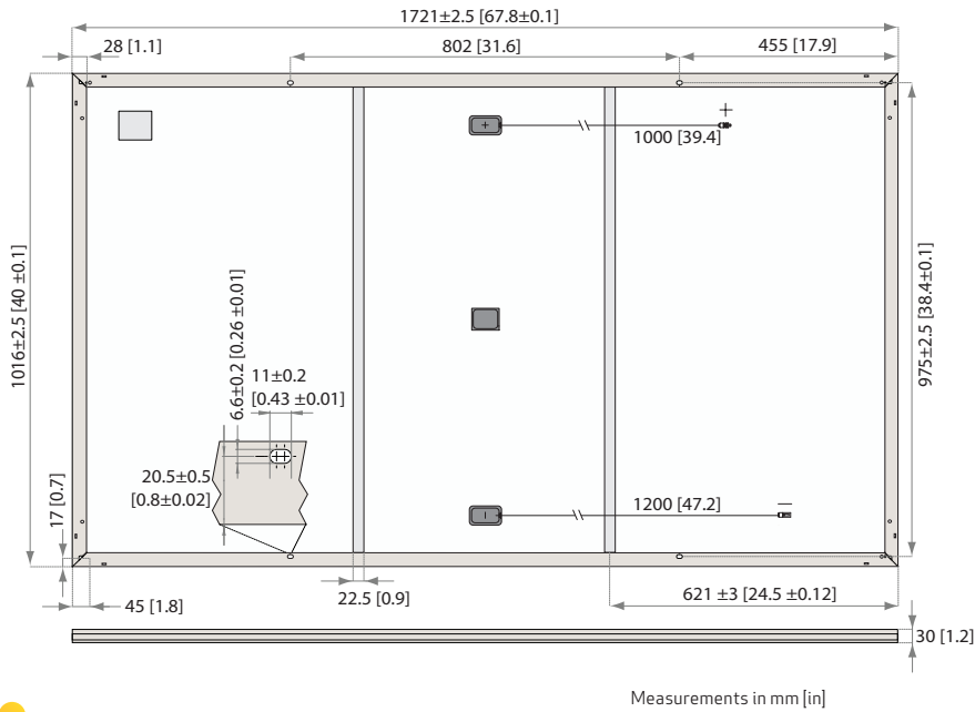
Fig. 14: Panel dimensions: REC Alpha Black Series
