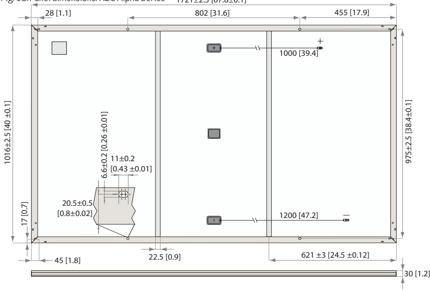
Fig. 13: Panel dimensions: REC Alpha Series 1721±2.5 [67.8±0.1]
