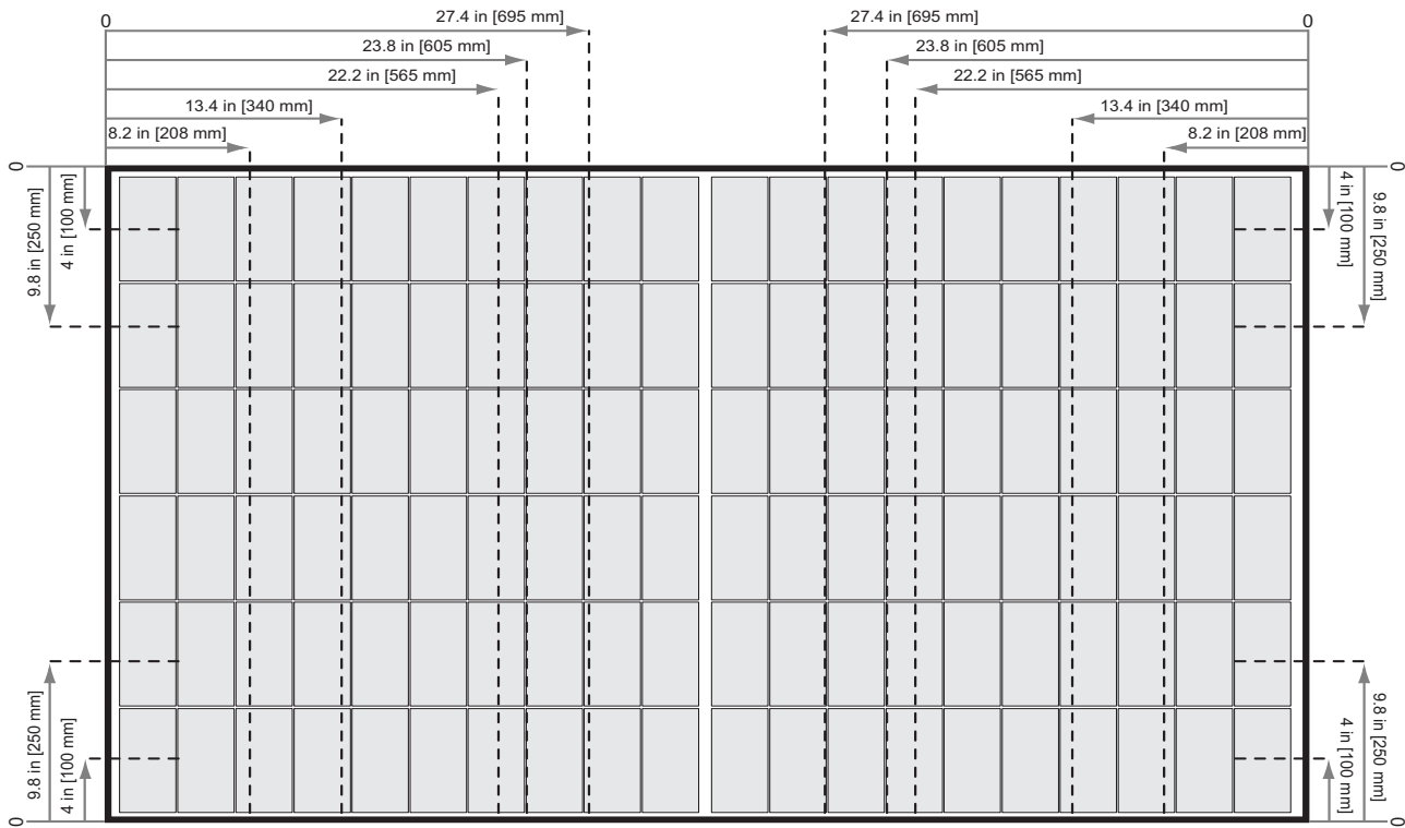
Fig. 3: Clamping of panels with rails parallel to short side of the module
