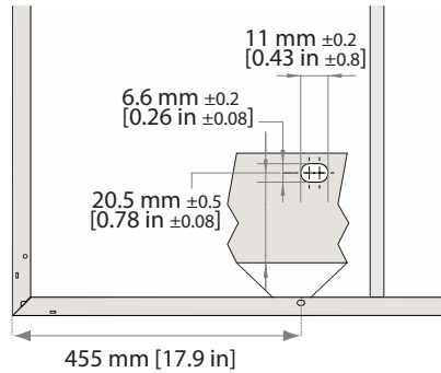
Fig. 6: Mounting holes: REC Alpha Series
